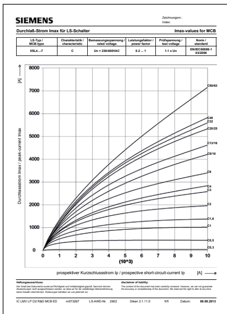
Figure 13: Cut-Off Characteristic I_c Displayed as a family of characteristics Valid for MCBs of series SSL4, C characteristic
