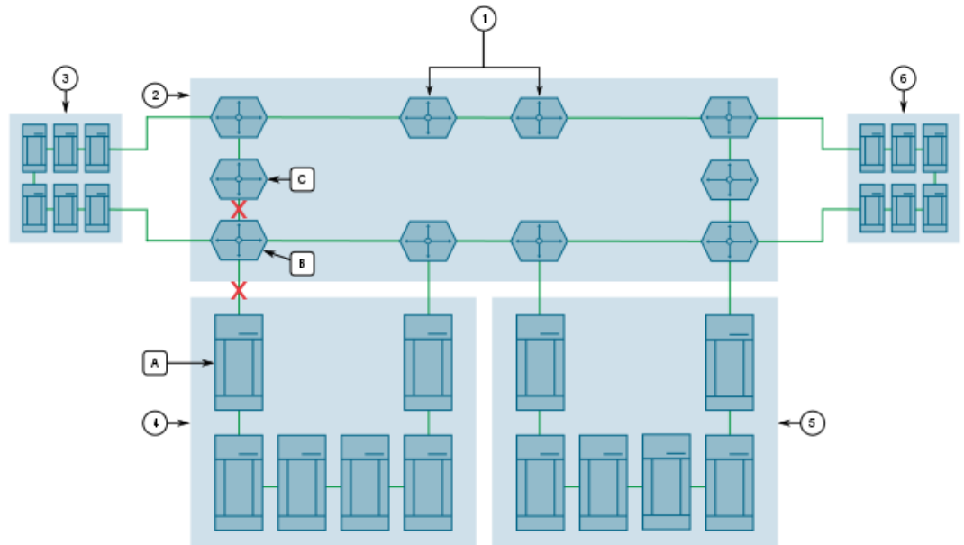
Figure 1: Sample Topology
