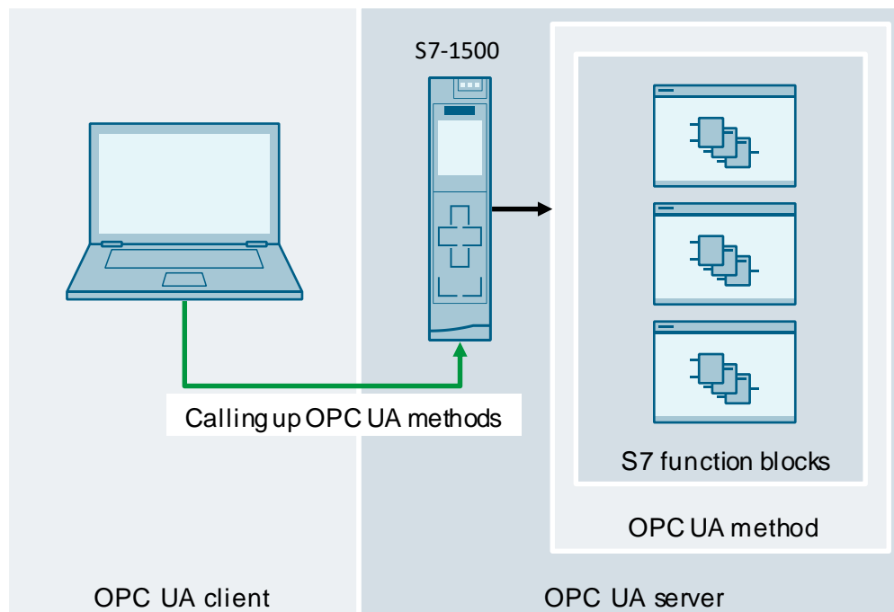
Figure 1-1 Pictorial schematic
