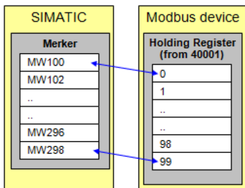
图 13-20 HR_Start_Offset_0
