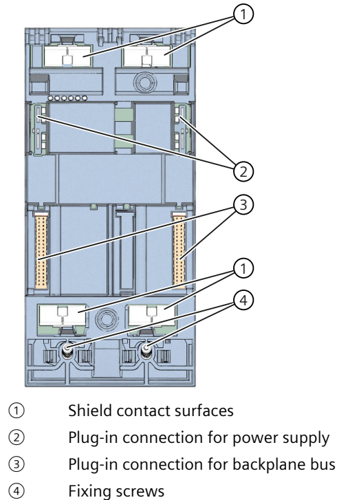
Figure 3-6 View of the CPU 1516-3 PN/DP - rear
