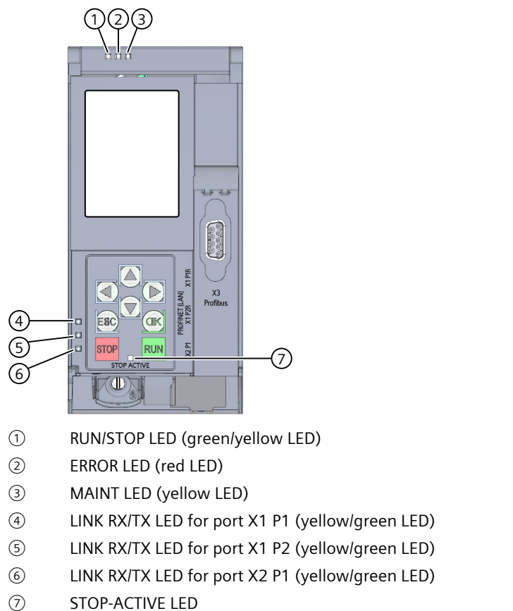
Figure 5-1 LED display of the CPU 1516-3 PN/DP (without front flap)
