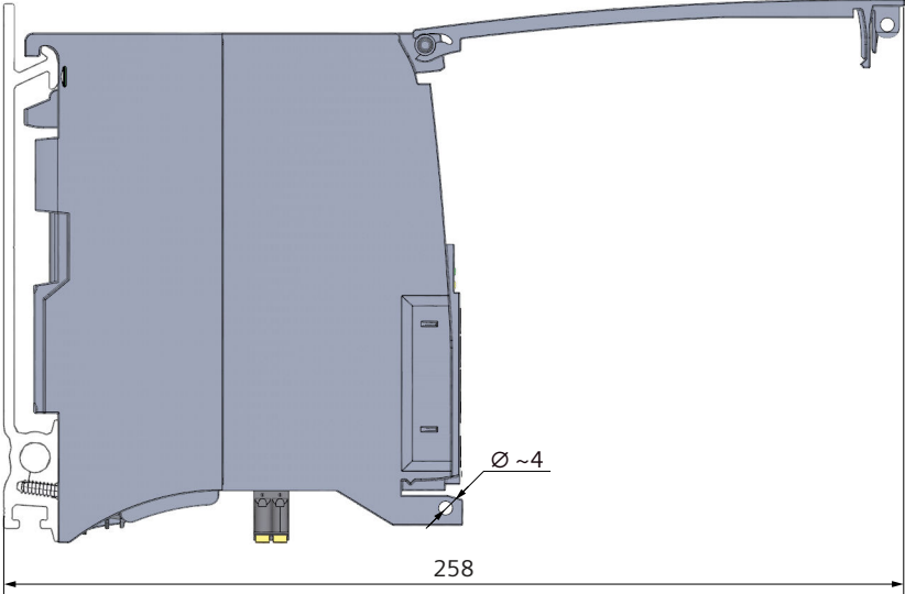
Figure A-2 CPU with open front panel
