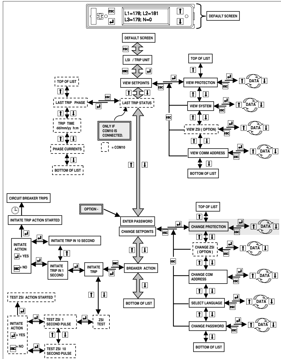
Figure 1-11: Detail of the menu for the overcurrent release LCD ETU 40
