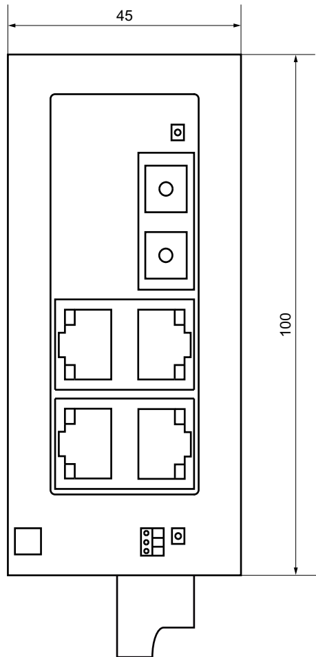
Figure 9-1 Dimension drawing, front view (example: SCALANCE XB004-1)
