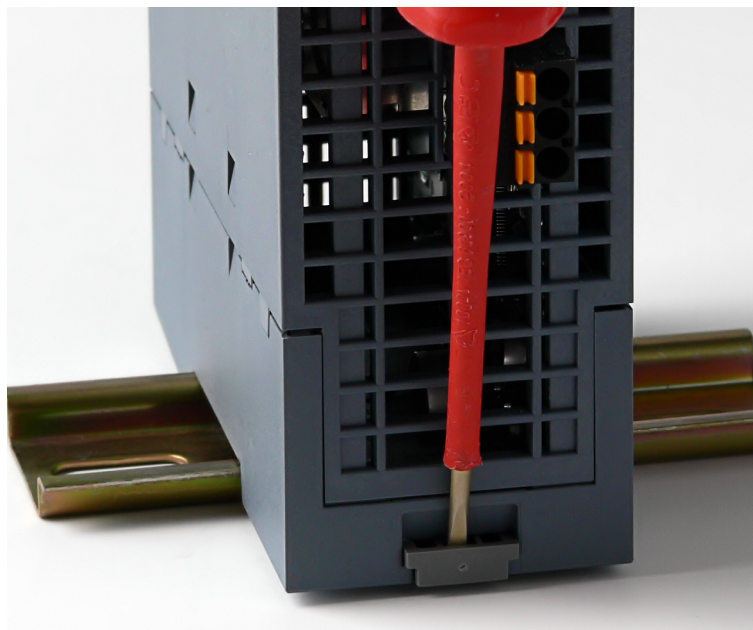
Figure 5-3 Removal from a 35 mm DIN rail
