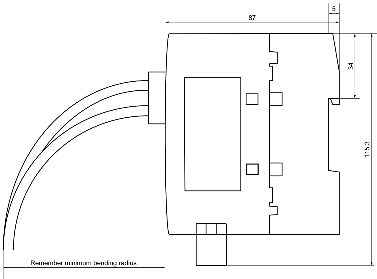
Figure 9-2 Dimension drawing, side view (example: SCALANCE XB004-1)
