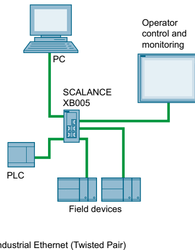
Figure 3-1 Example of an electrical star topology with SCALANCE XB005
