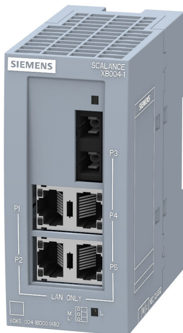
Figure 4-1 SCALANCE XB004-1
