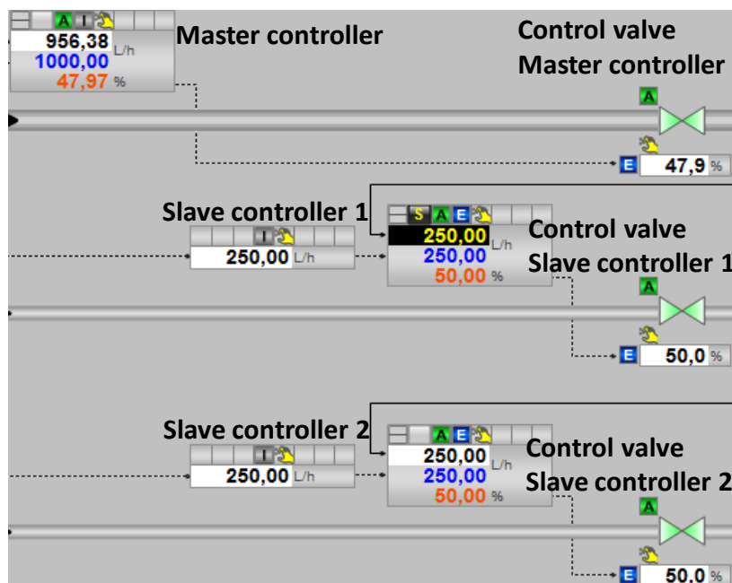
Faulty slave controller
