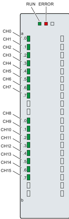
Figure 5-1 LED displays of the module DI 16x24VDC SRC BA
