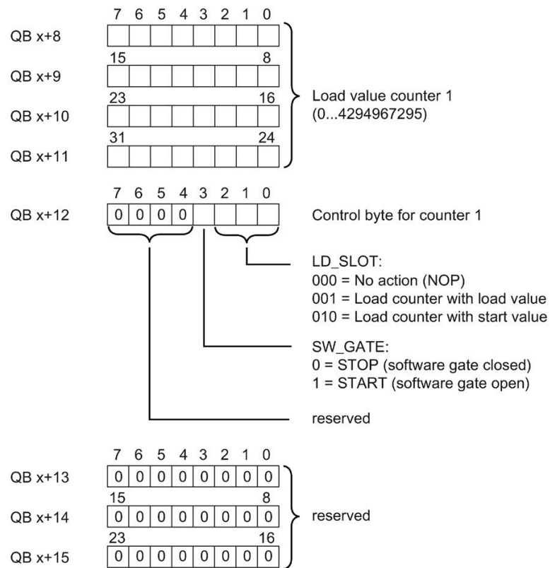
Figure 4-6 Assignment of the address space of the control interface of the DI 32x24VDC Count (bytes 8 to 15)
