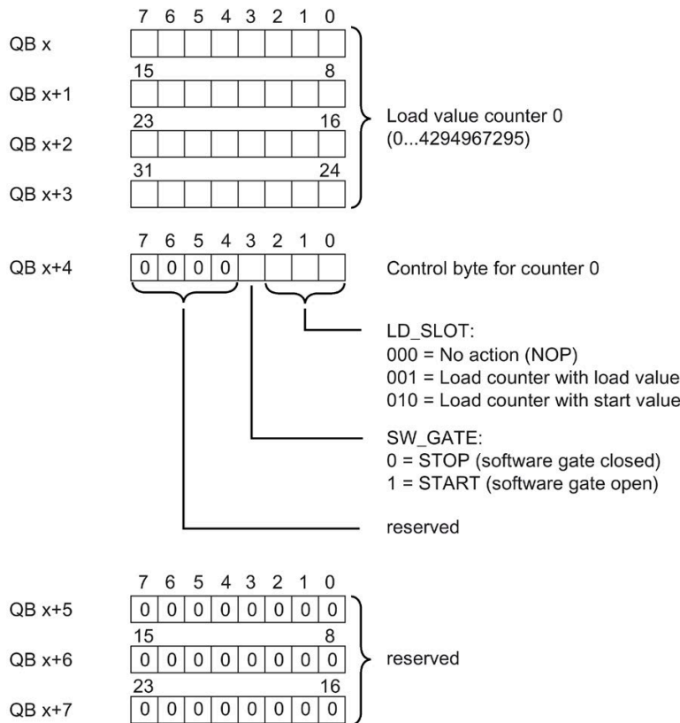
Figure 4-5 Assignment of the address space of the control interface of the DI 32x24VDC Count (bytes 0 to 7)
