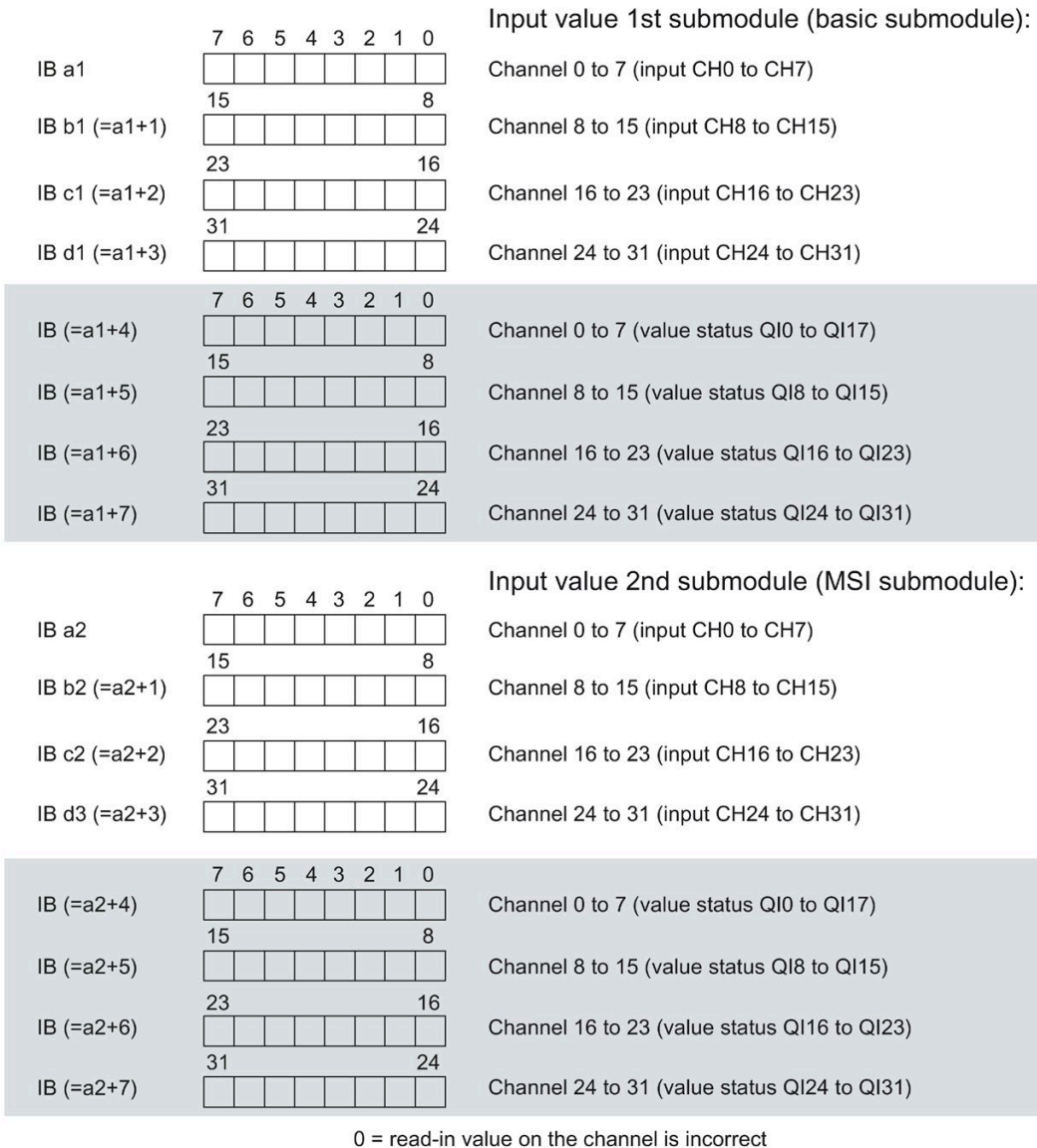
Figure 4-3 Address space for configuration as 1 x 32-channel DI 32x24VDC HF MSI with value status
