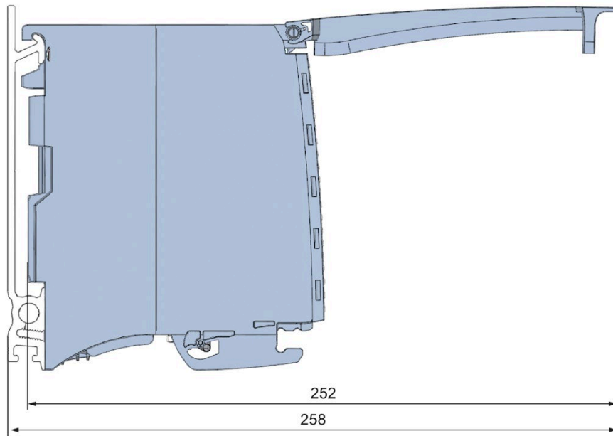
Figure A-2 Dimensional drawing of the DI 32x24VDC HF module, side view with open front cover
