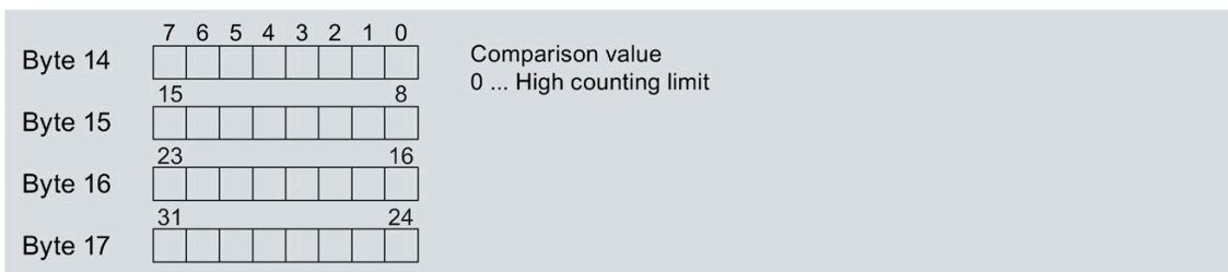
Figure B-3 Structure of data record 0: Bytes 5 to 17
