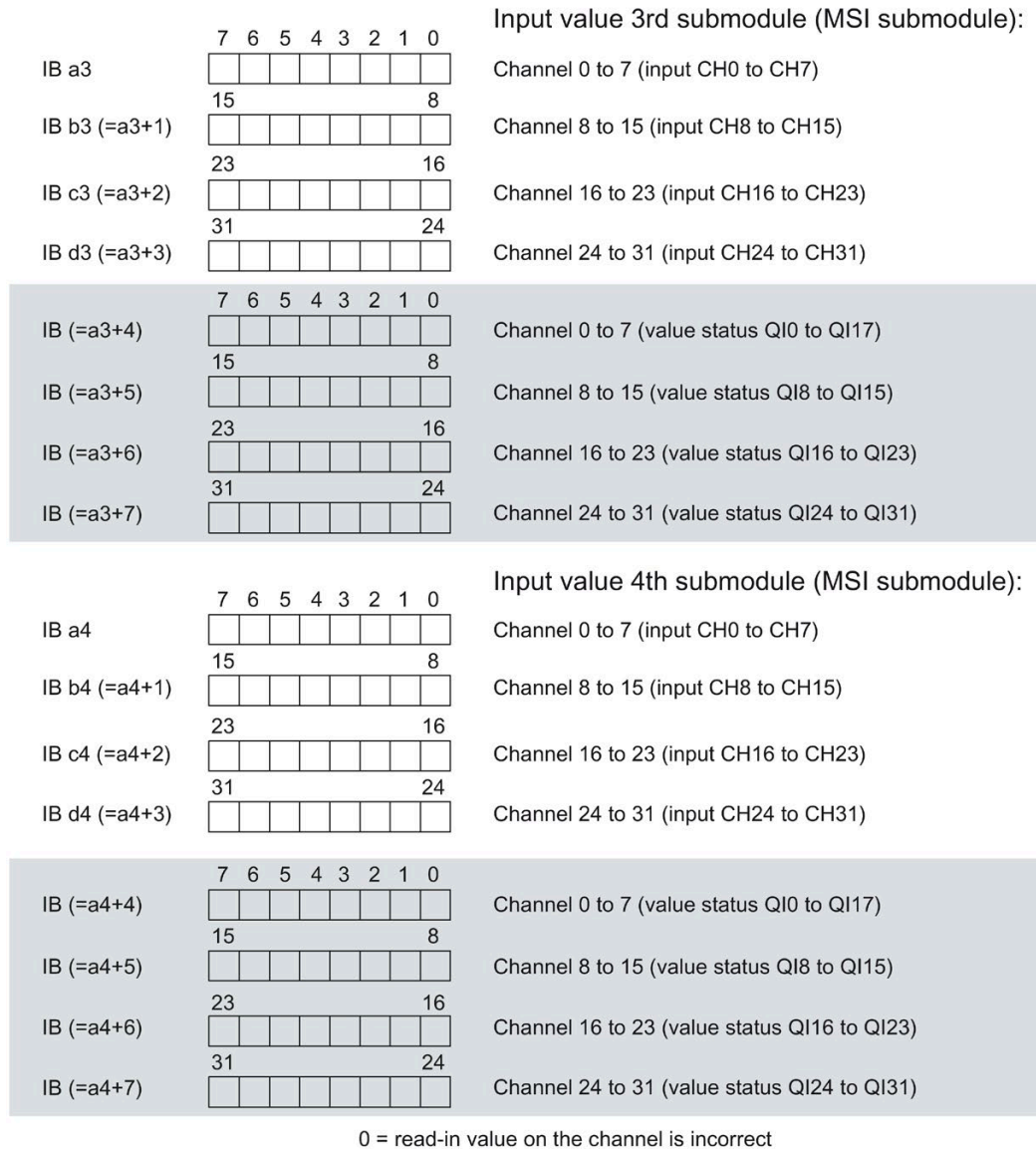
Figure 4-4 Address space for configuration as 1 x 32-channel DI 32x24VDC HF MSI with value status
