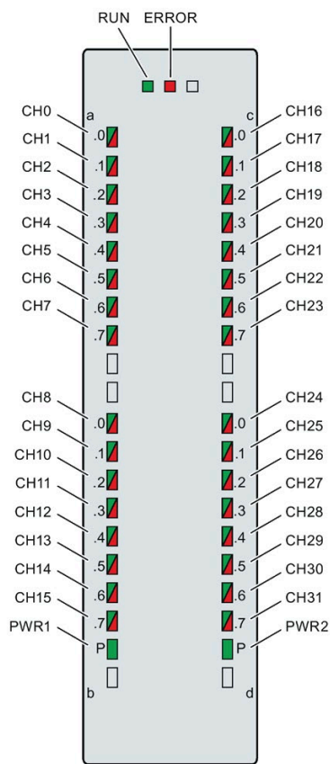
Figure 5-1 LED displays of the module DI 32x24VDC HF
