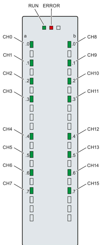
Figure 5-1 LED displays of the module DI 16x230VAC BA
