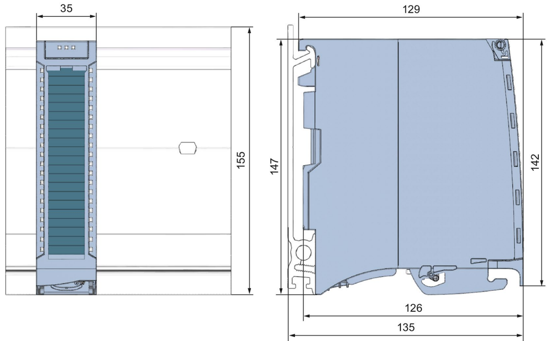
Figure A-1 Dimensional drawing of the DI 16x24VAC BA module
