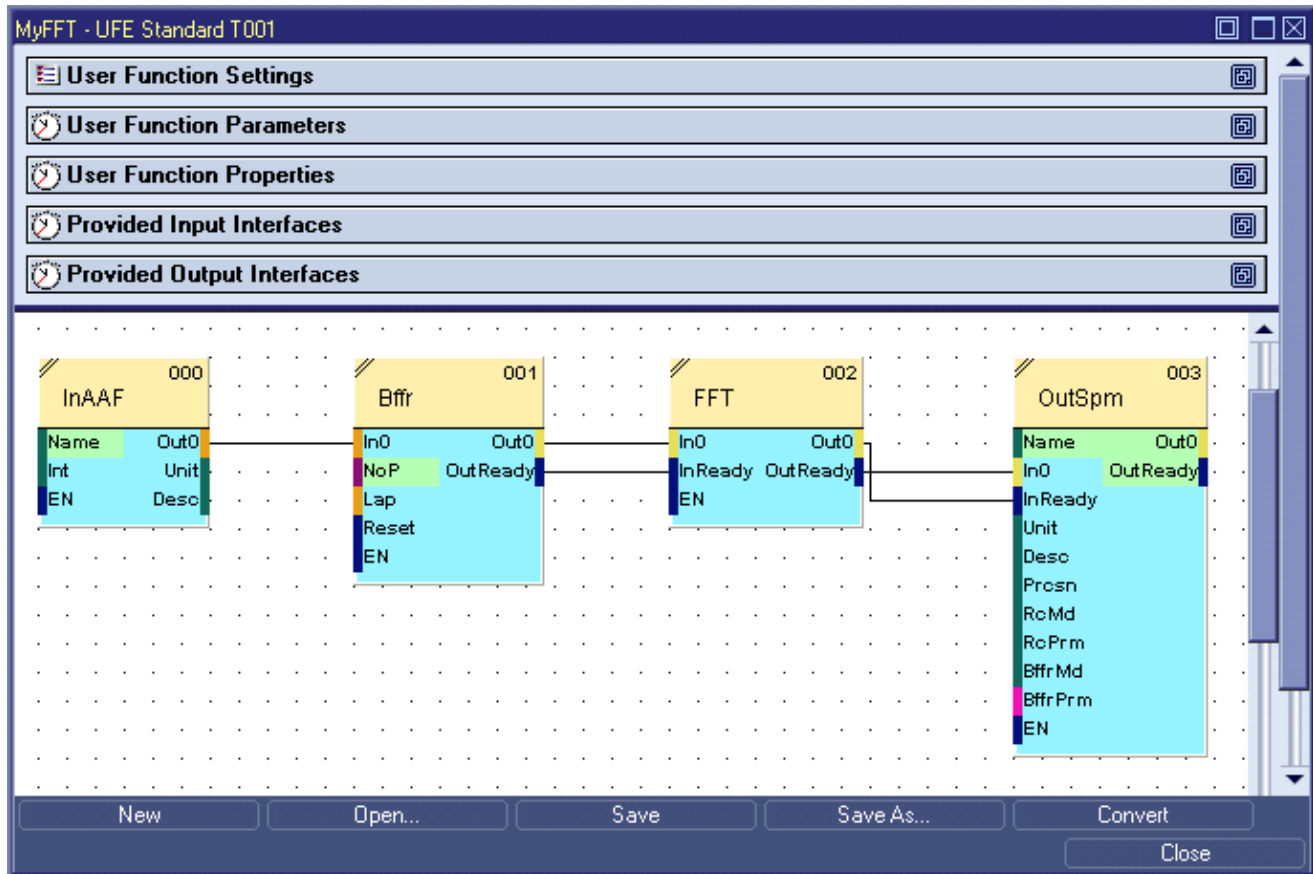
Figure 10: Example of a UFE Standard T001
