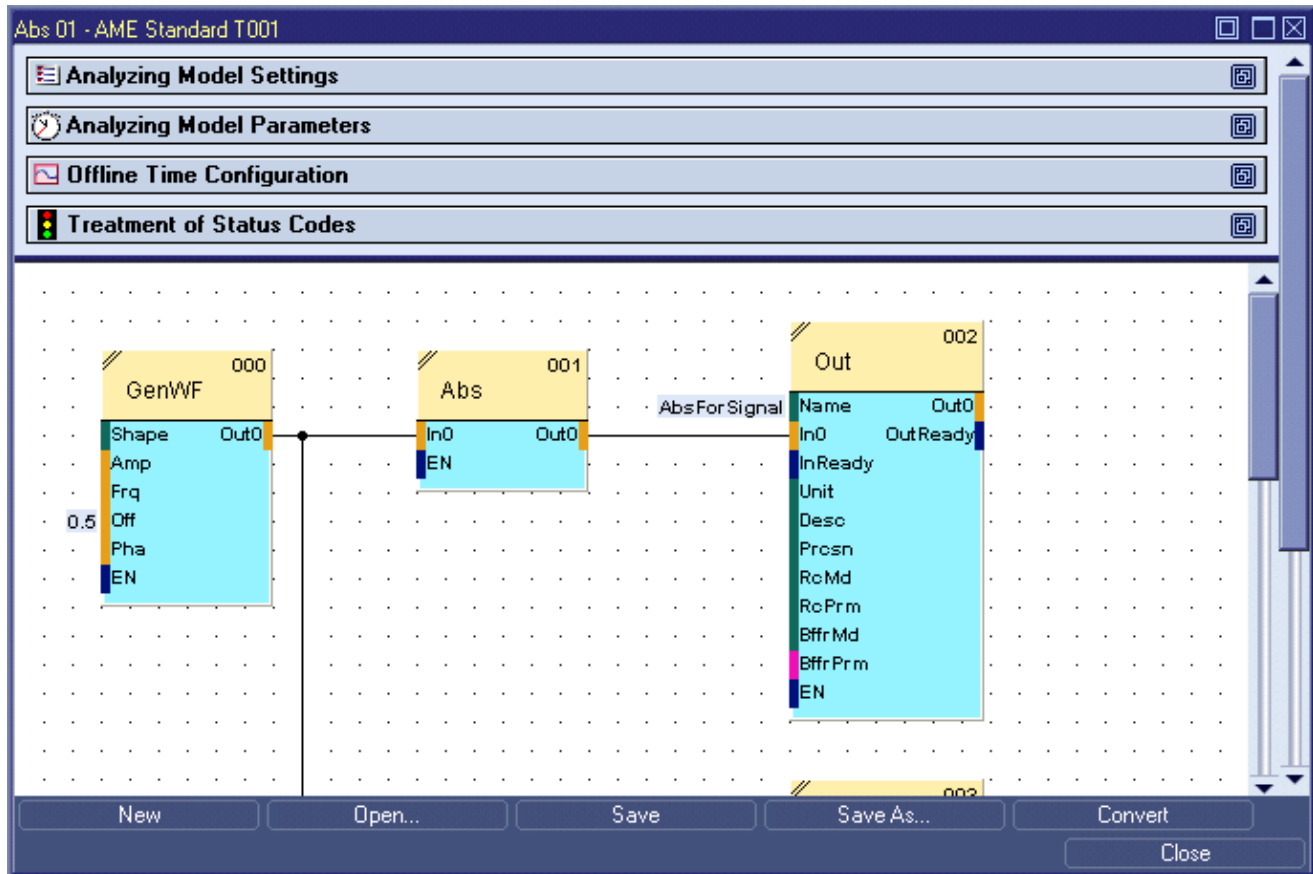
Figure 4: Example of an AME Standard T001
