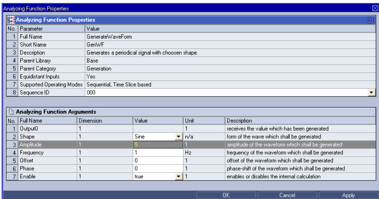
Figure 8: Example of an Analyzing Function Properties Dialog
