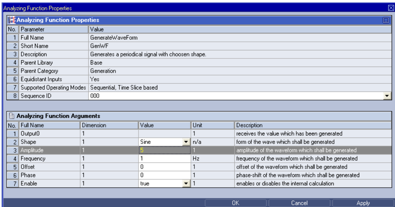
Figure 14: Example of an Analyzing Function Properties Dialog
