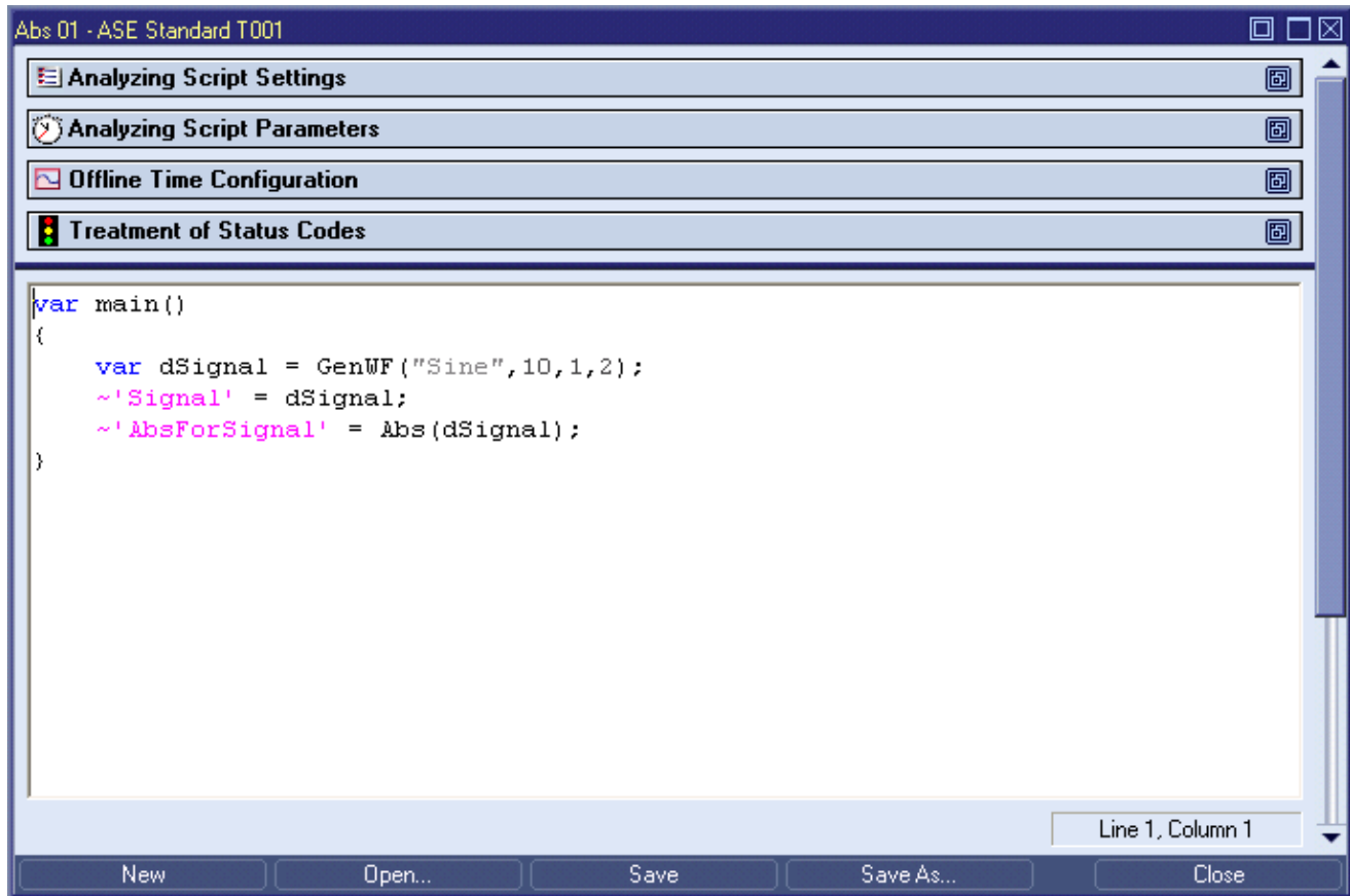
Figure 9: Example of an ASE Standard T001
