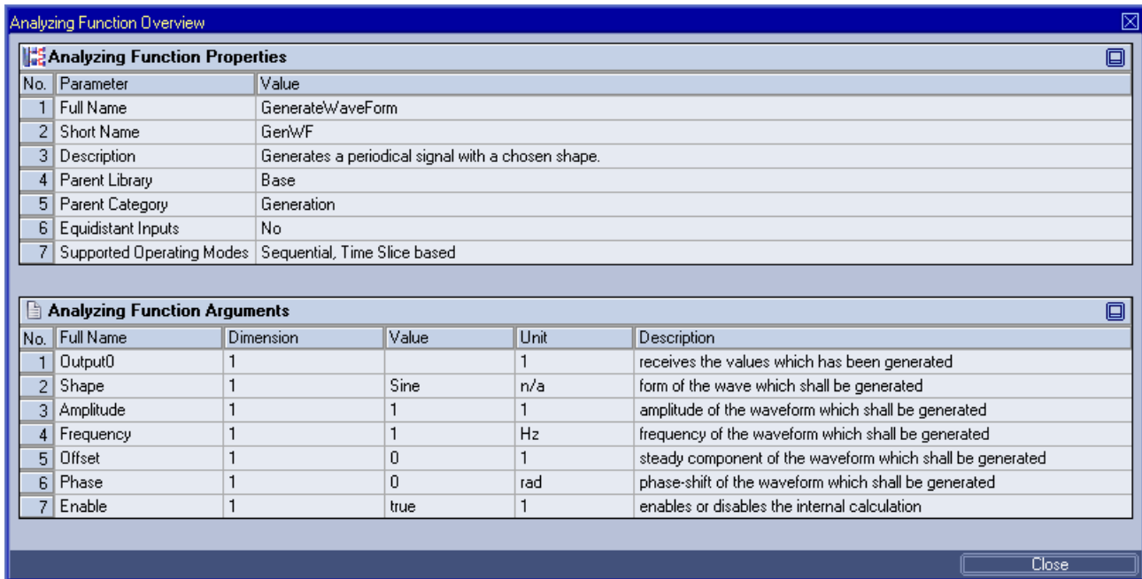
Figure 2: Example of an Analyzing Function Overview Dialog
