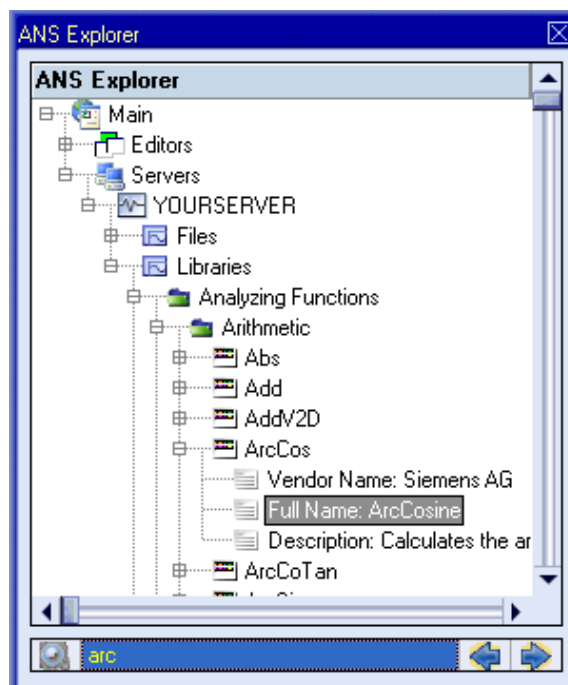
Figure 3: Example of a Search Area within the ANS Explorer
