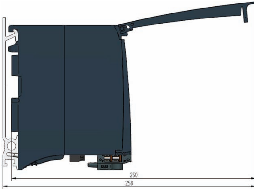
Figure A-2 Dimension drawing of the PM 70 W 120/230VAC load power supply module, side view with the front cover open
