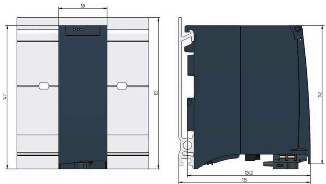
Figure A-1 Dimension drawing of the PM 70 W 120/230 VAC load power supply module
