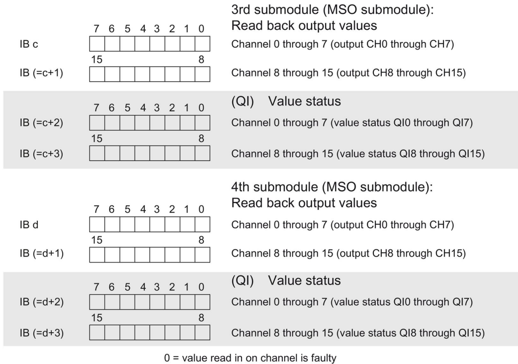
Figure 4-4 Address space for configuration as 1 x 16-channel DQ 16x24VDC/0.5A BA MSO with value status
