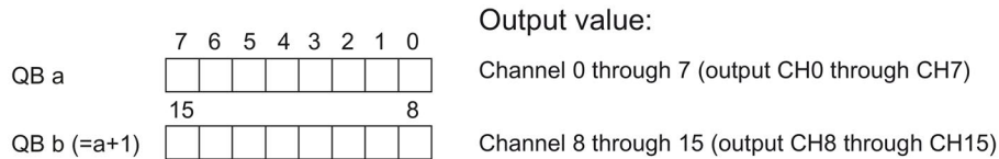
Figure 4-1 Address space for configuration as 1 x 16-channel DQ 16x24VDC/0.5A BA
