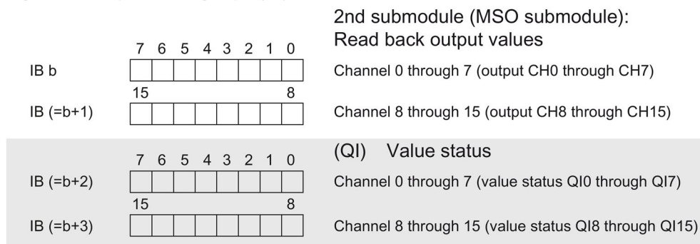
Figure 4-3 Address space for configuration as 1 x 16-channel DQ 16x24VDC/0.5A BA MSO with value status
