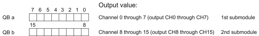
Figure 4-2 Address space for configuration as 2 x 8-channel DQ 32x24VDC/0.5A BA S
