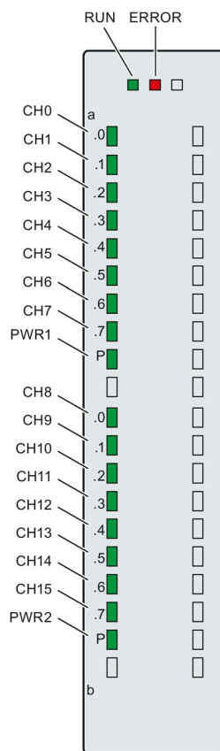
Figure 5-1 LED displays of the module DQ 16x24VDC/0.5A BA
