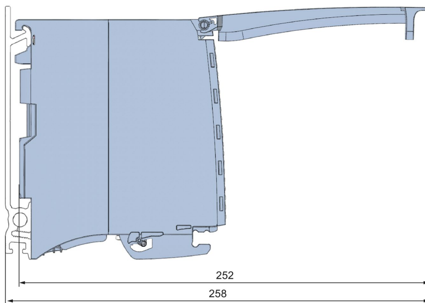
Figure A-2 Dimensional drawing of the DQ 16x24VDC/0.5A BA module, side view with open front cover
