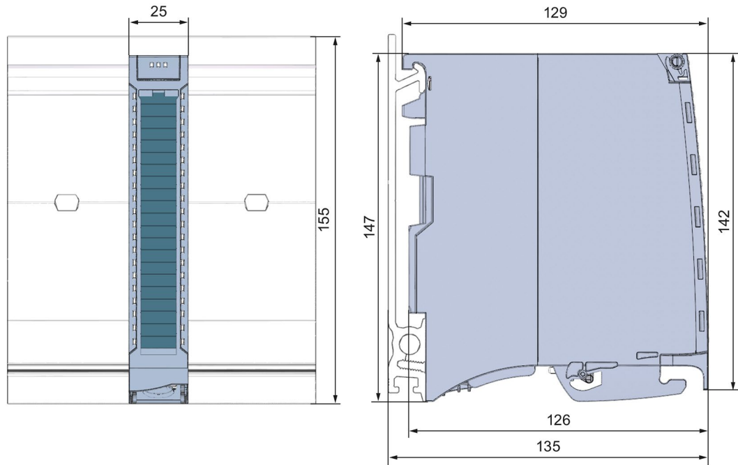
Figure A-1 Dimensional drawing of the DQ 16x24VDC/0.5A BA module
