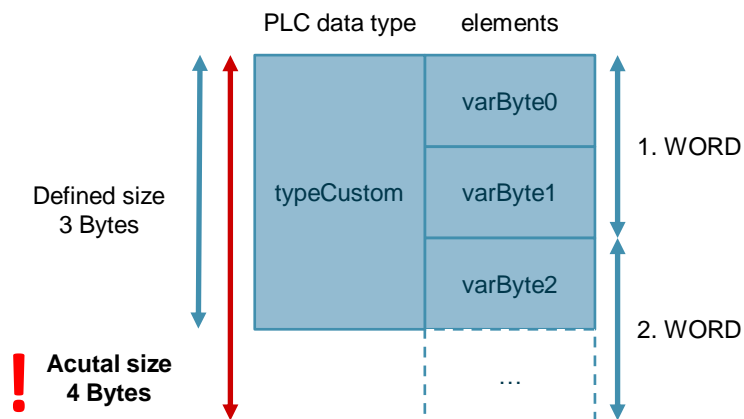
Figure 3-33: PLC data types always end at WORD limits
