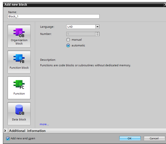
Figure 3-5: "Add new block" dialog (FC)
