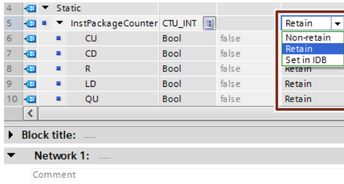
Figure 3-27: Retentive counter as multi-instance
