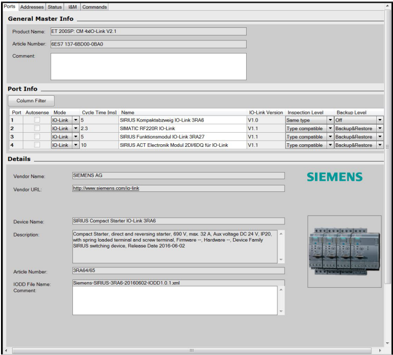
Figure 1-5 S7-PCT with IODD of a device and the device information contained therein
